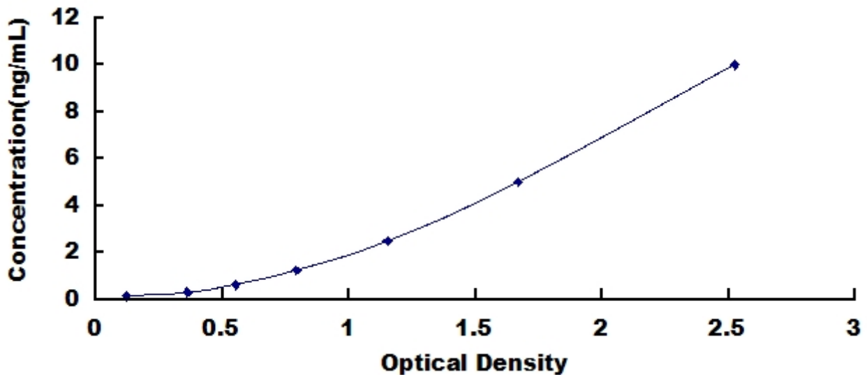
Typical Standard Curve for ACVR2B, Human ELISA.
