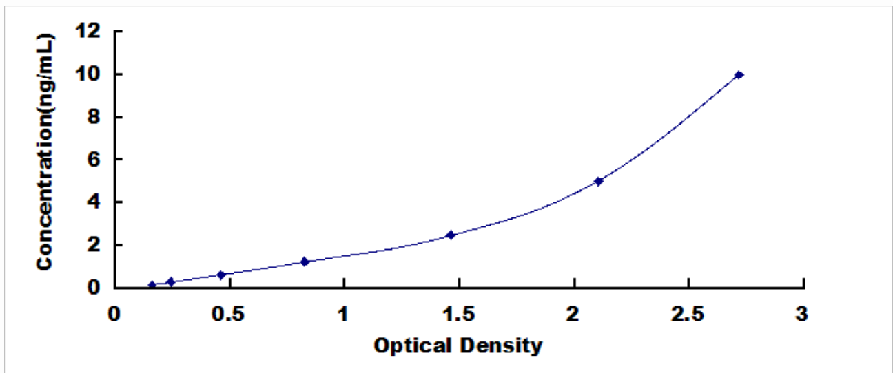
Typical Standard Curve for Adiponectin, Mouse ELISA.
