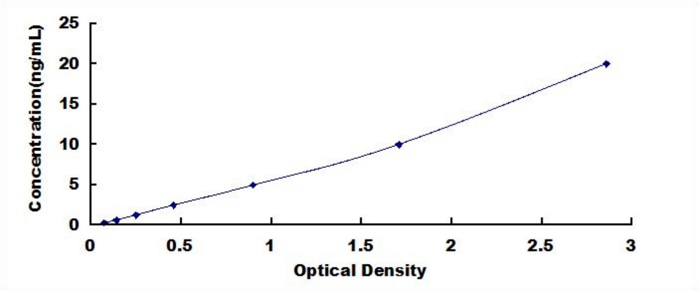
Typical Standard Curve for ADRbK1, Human ELISA.
