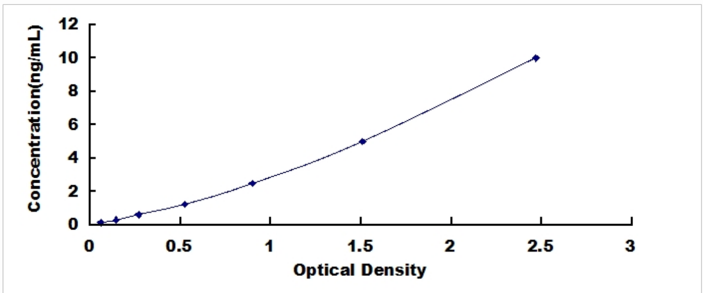
Typical Standard Curve for AAP, Rat ELISA.
