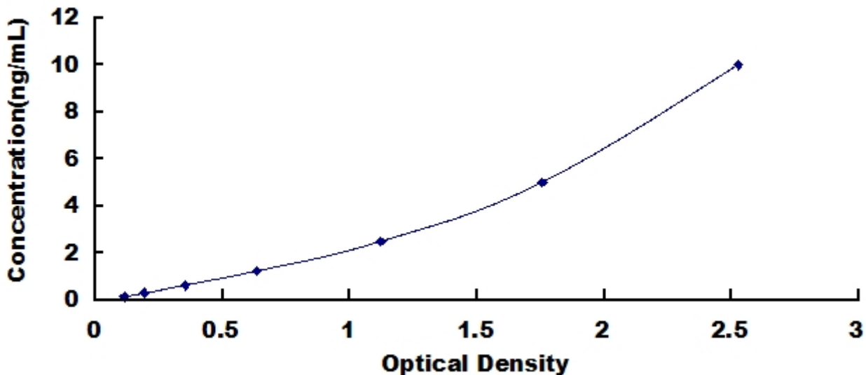
Typical Standard Curve for ARL1, Human ELISA.
