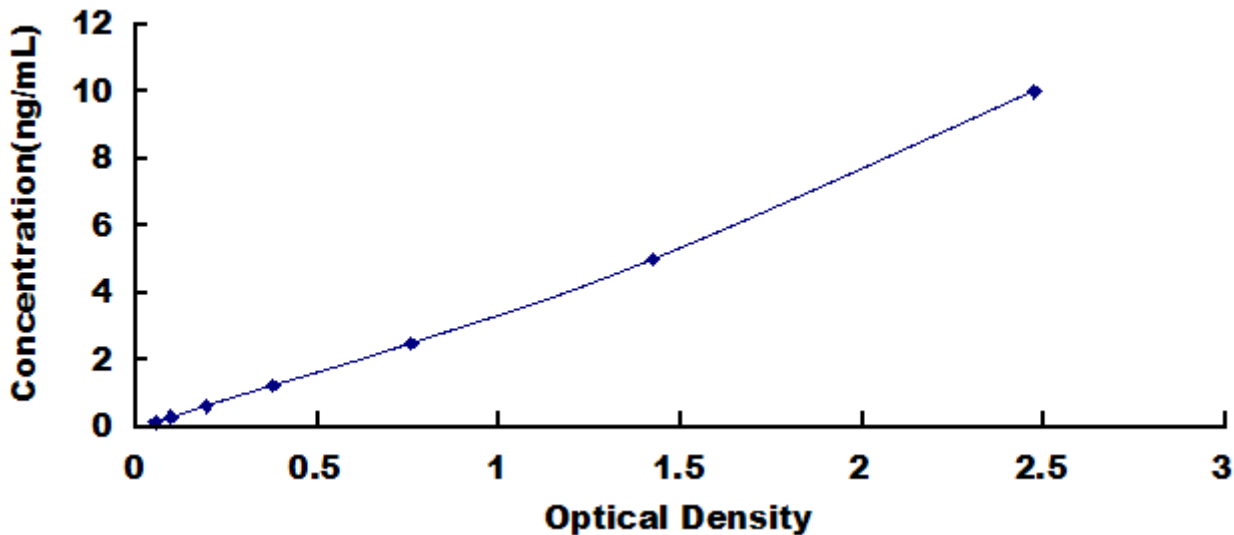
Typical Standard Curve for RNPEP, Human ELISA.
