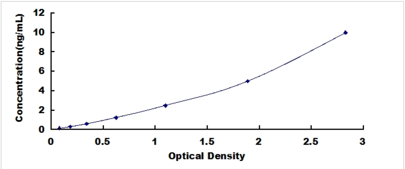
Typical Standard Curve for Angiotstatin, Rat ELISA.
