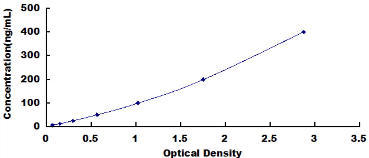
Typical Standard Curve for APOA1, Human ELISA.
