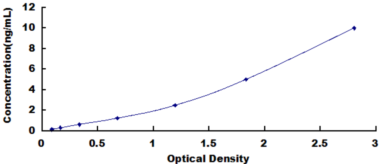
Typical Standard Curve for APAF1, Mouse ELISA.
