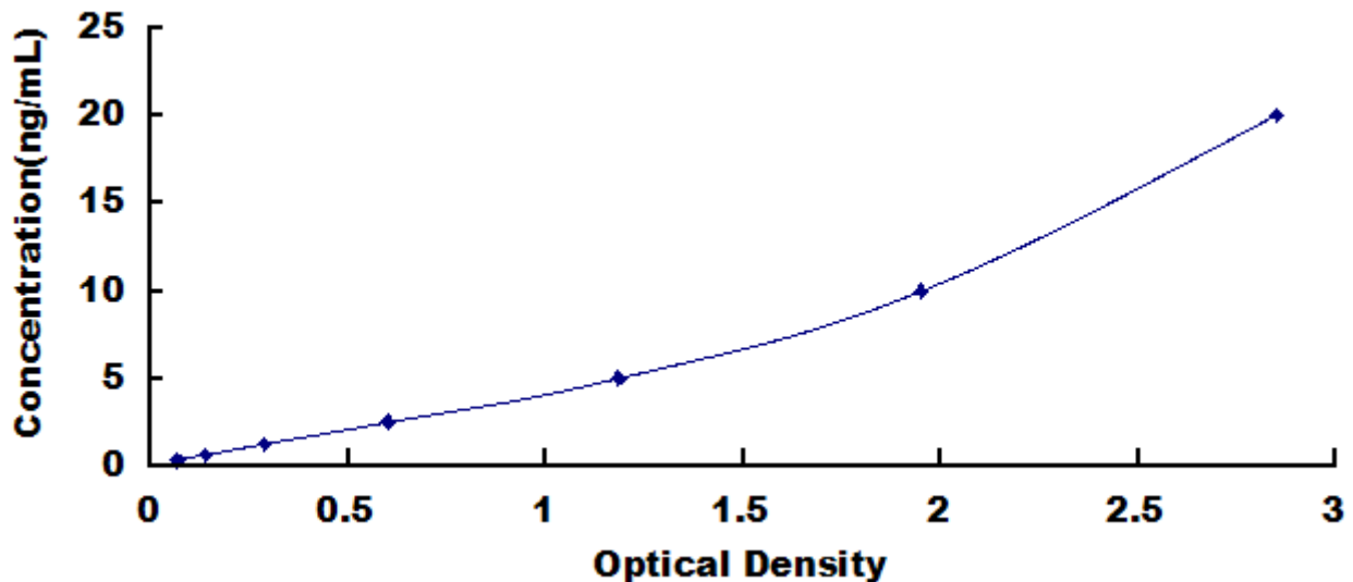
Typical Standard Curve for AMFR, Human ELISA.
