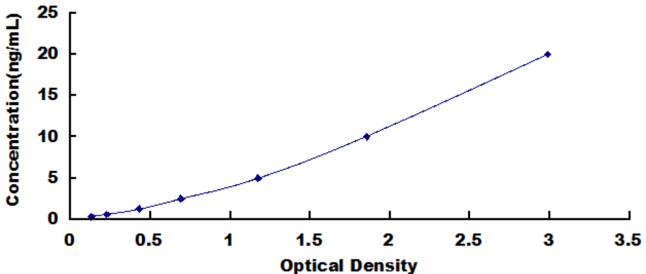
Typical Standard Curve for Brevican, Human ELISA.
