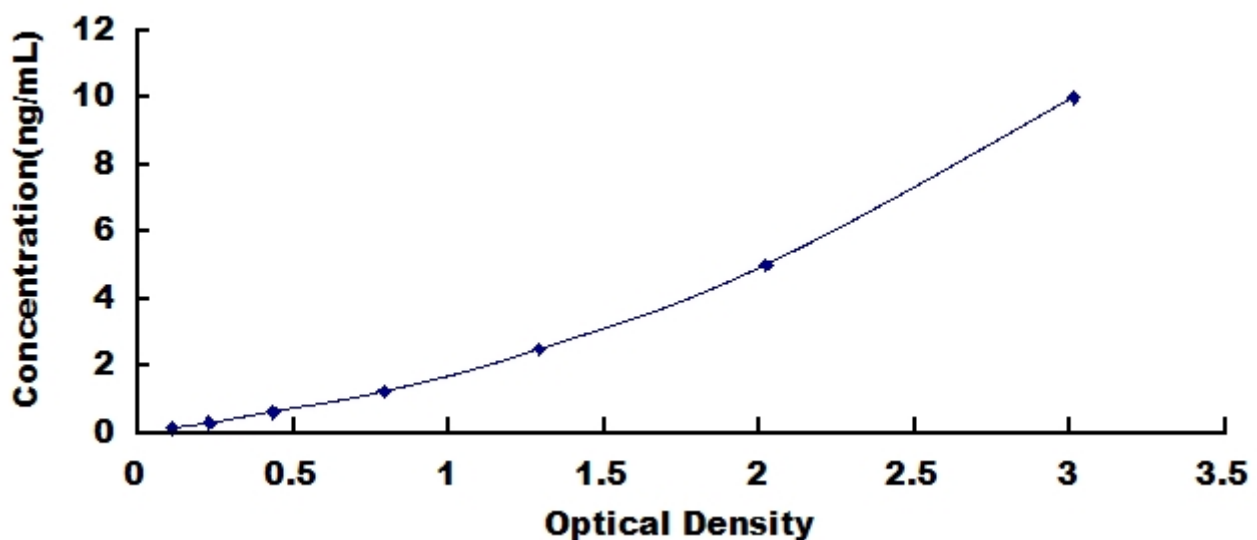
Typical Standard Curve for C1QTNF3, Human ELISA.
