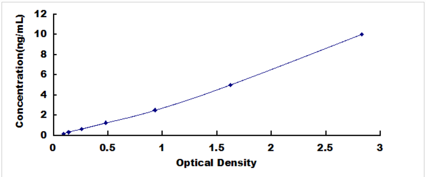
Typical Standard Curve for CEBPa, Human ELISA.
