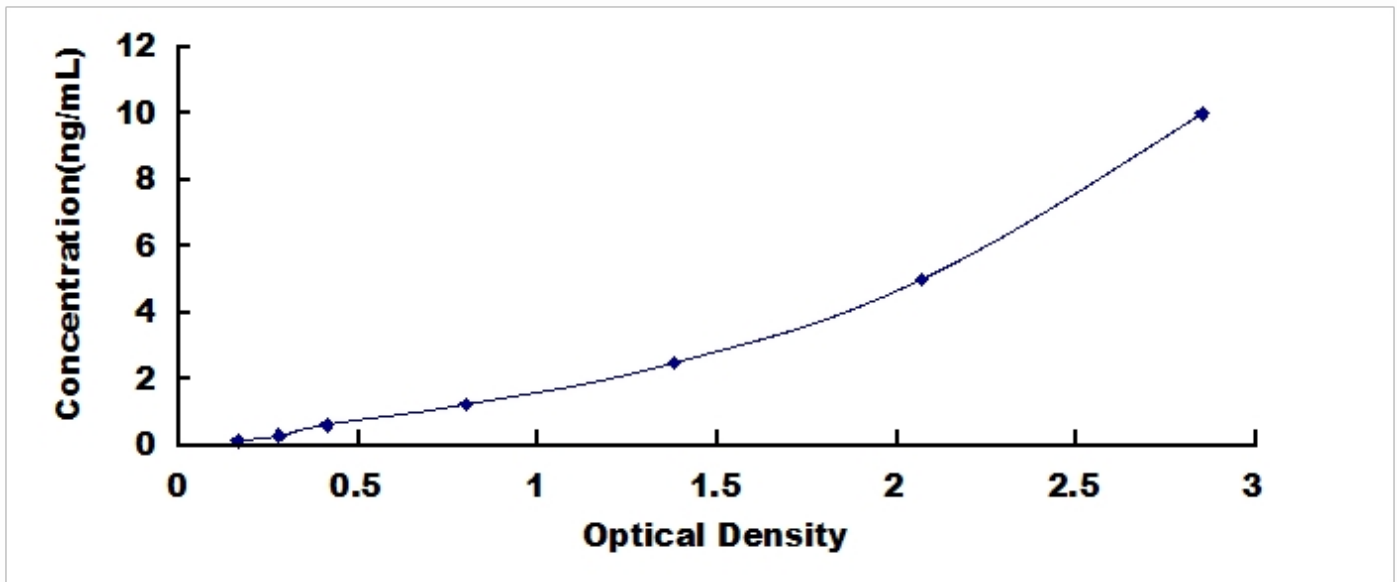
Typical Standard Curve for CELF1, Human ELISA.
