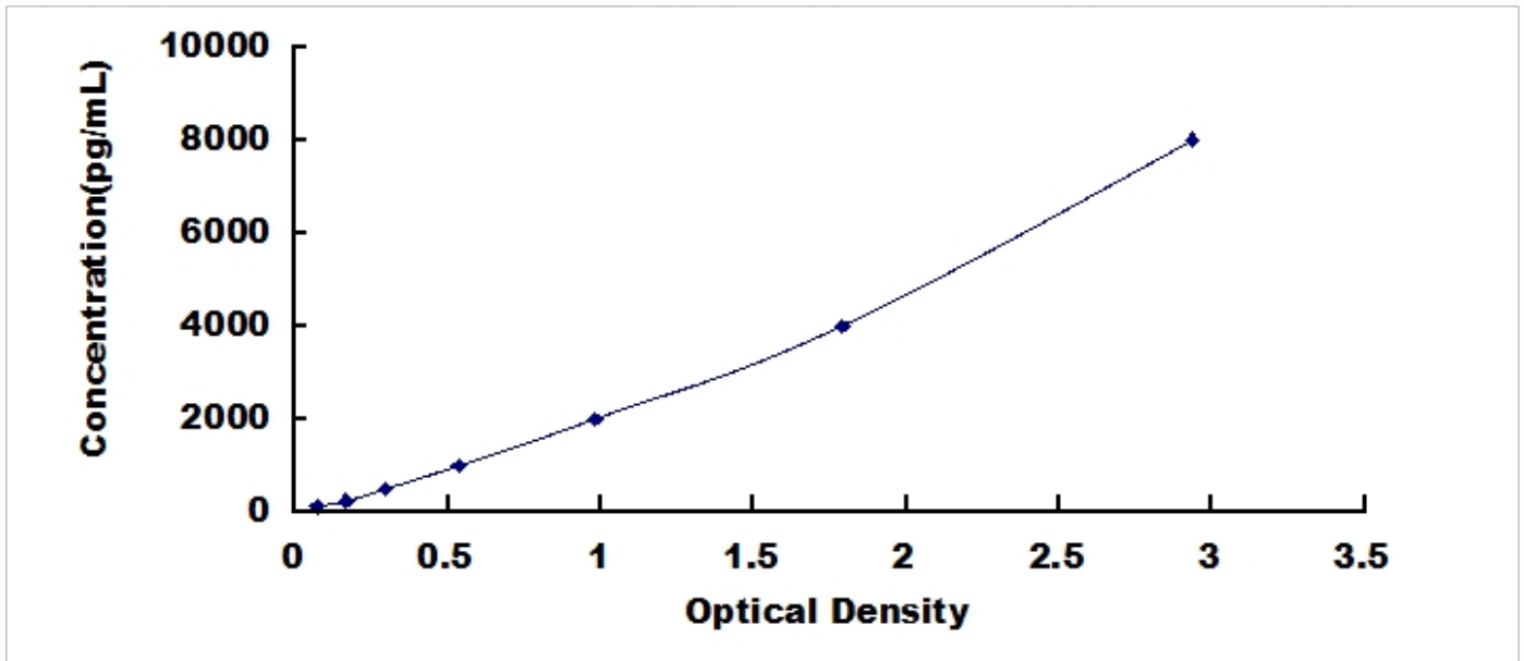
Typical Standard Curve for CAMP, Rat ELISA.
