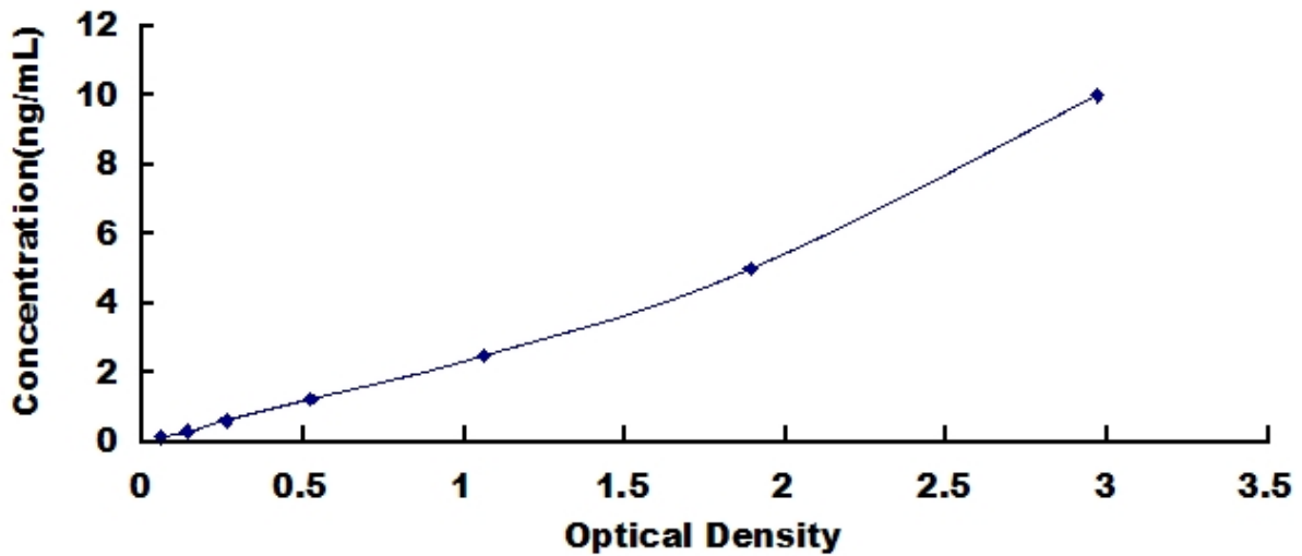
Typical Standard Curve for CDC25, Human ELISA.
