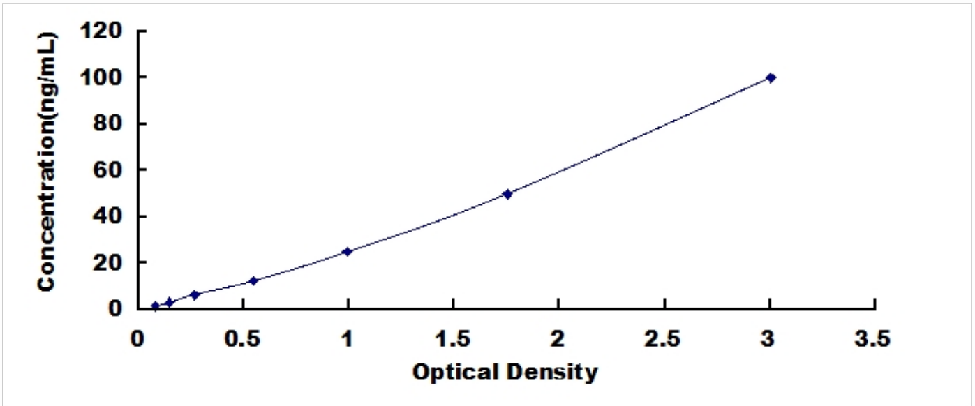
Typical Standard Curve for PRSS8, Human ELISA.
