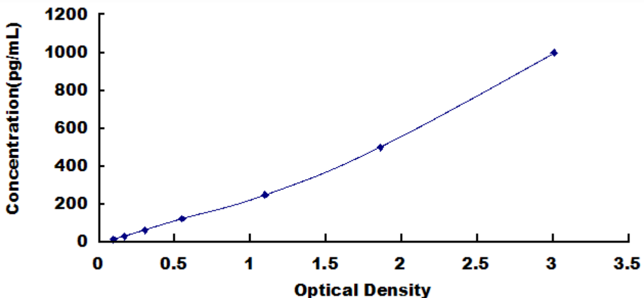
Typical Standard Curve for bTG, Human ELISA.
