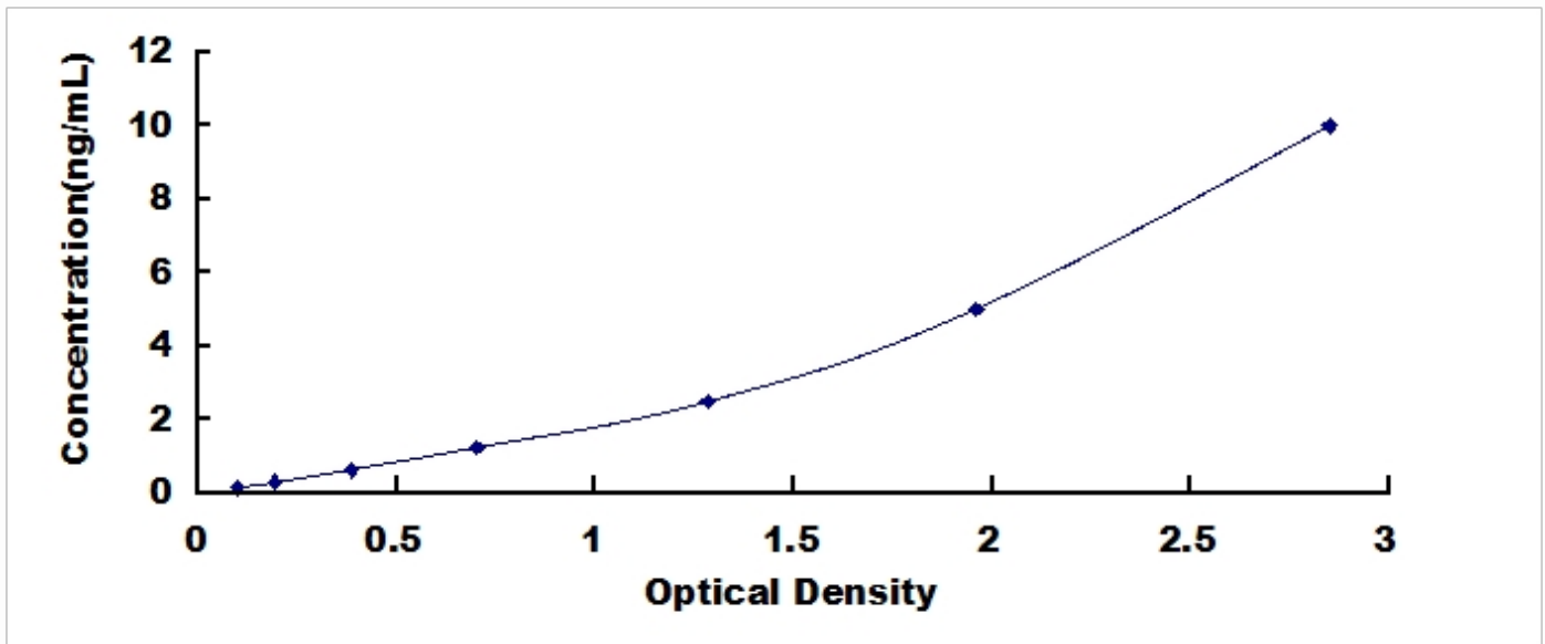
Typical Standard Curve for CX3CR1, Human ELISA.
