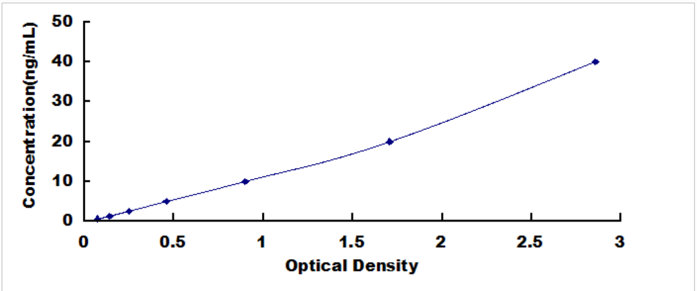
Typical Standard Curve for CHGB, Human ELISA.
