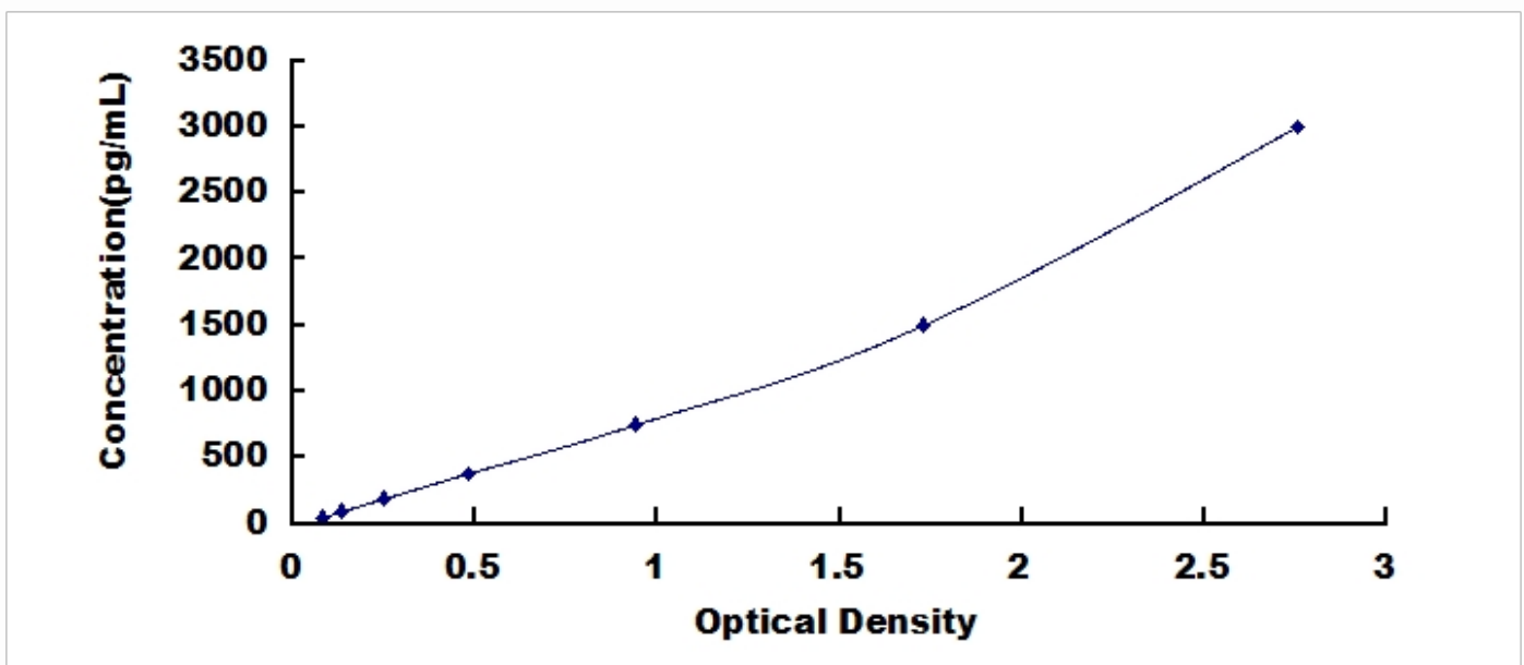
Typical Standard Curve for CD83, Mouse ELISA.
