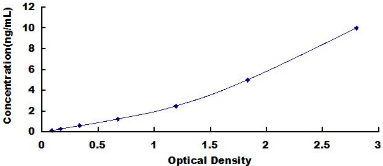
Typical Standard Curve for CD8a, Human ELISA.
