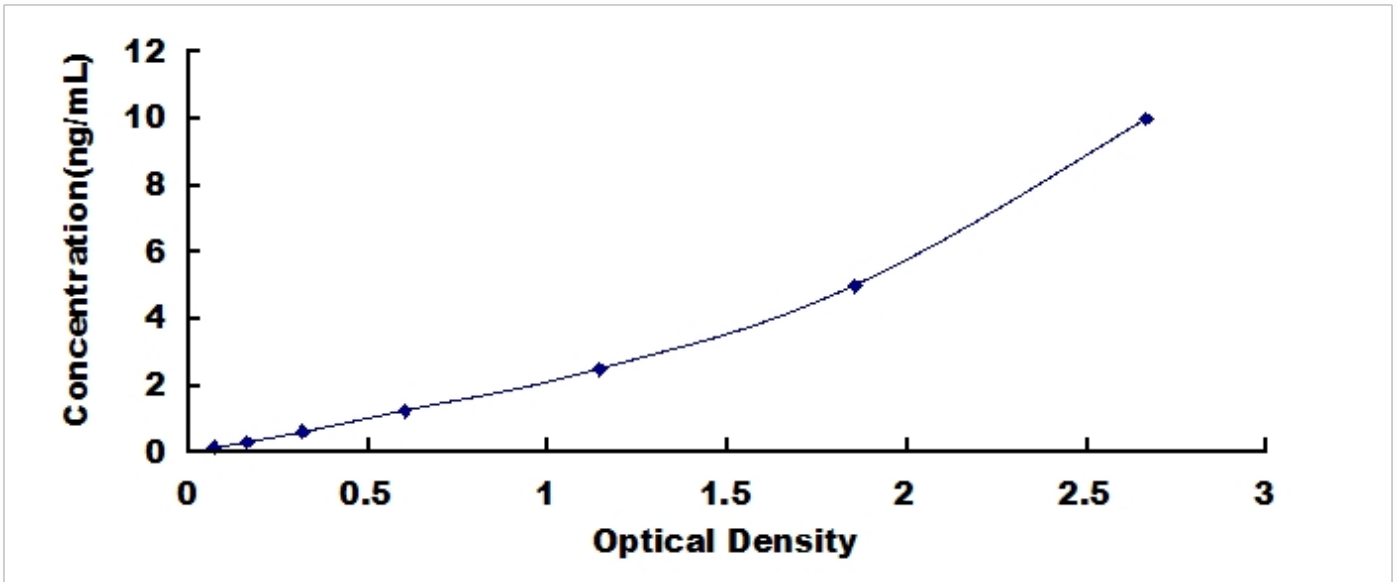
Typical Standard Curve for CCDC80, Human ELISA.
