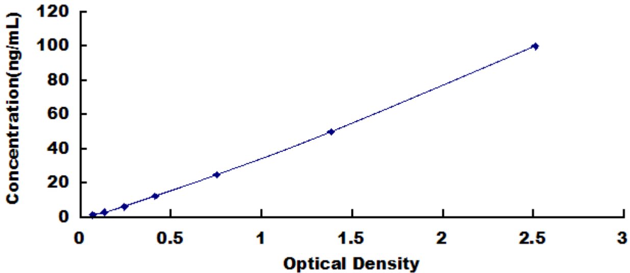
Typical Standard Curve for COL3, Equine ELISA.
