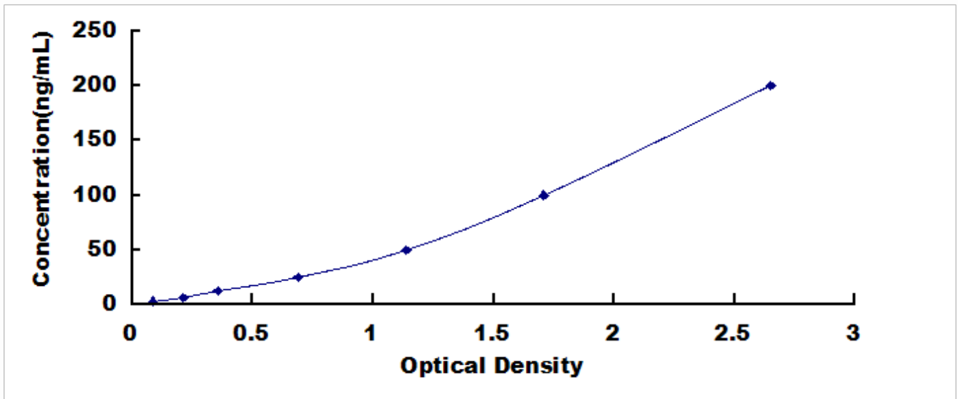
Typical Standard Curve for COL4a4, Human ELISA.
