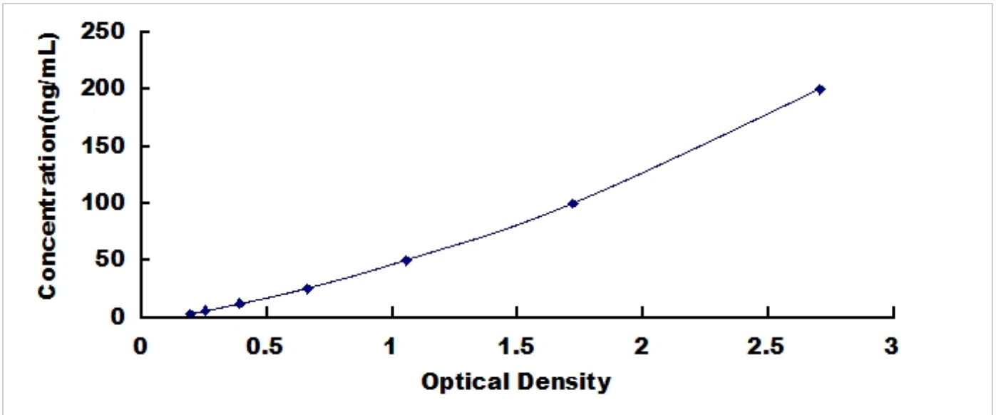
Typical Standard Curve for COL5, Human ELISA.
