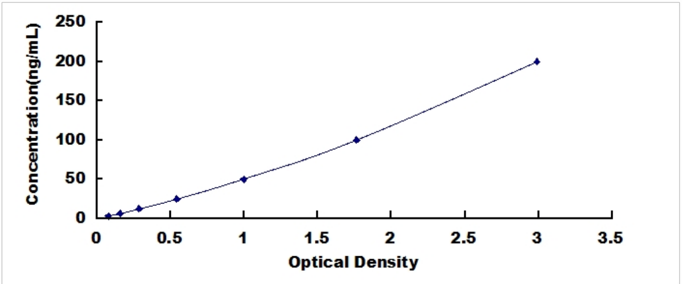
Typical Standard Curve for COL10, Mouse ELISA.
