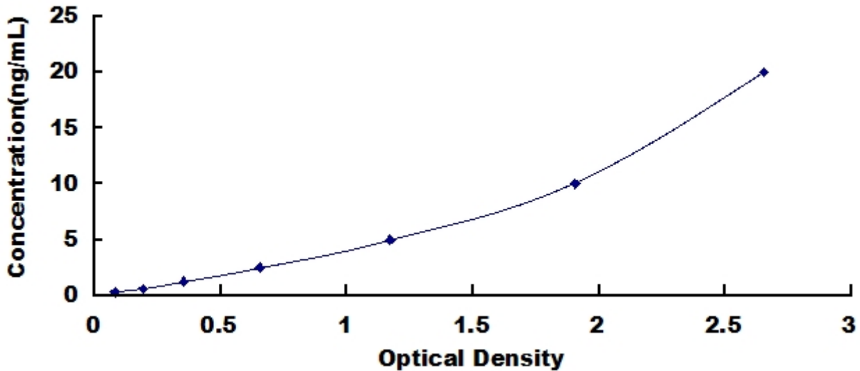
Typical Standard Curve for C5aR1, Human ELISA.
