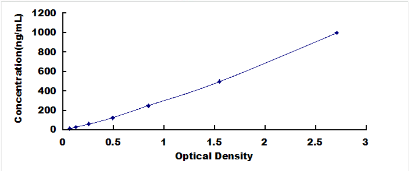
Typical Standard Curve for CFH, Human ELISA.
