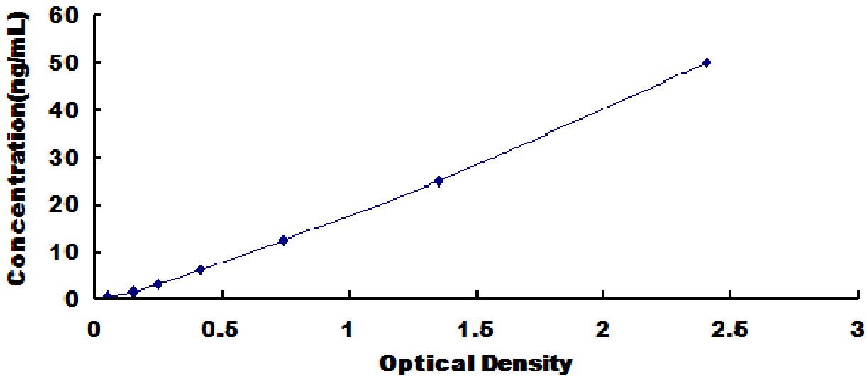
Typical Standard Curve for CF6, Rat ELISA.
