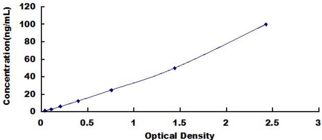
Typical Standard Curve for CKM, Human ELISA.
