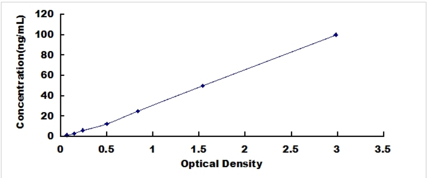
Typical Standard Curve for CKM, Porcine ELISA.
