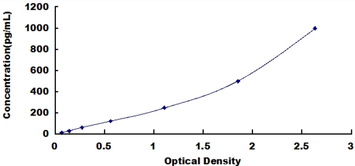
Typical Standard Curve for CCND2, Human ELISA.
