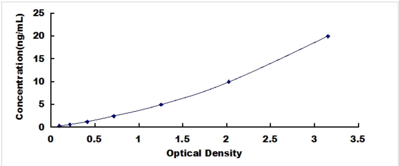
Typical Standard Curve for CDK8, Human ELISA.
