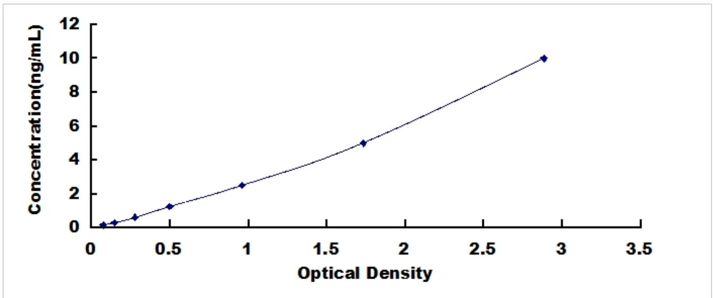
Typical Standard Curve for CST1, Human ELISA.
