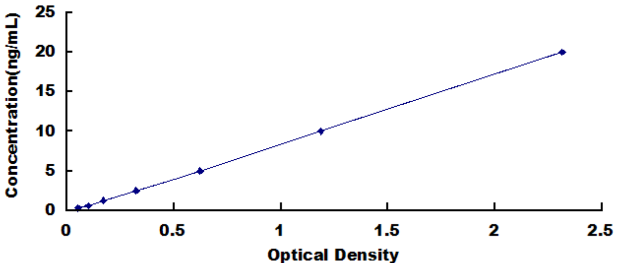
Typical Standard Curve for CYBb, Mouse ELISA.
