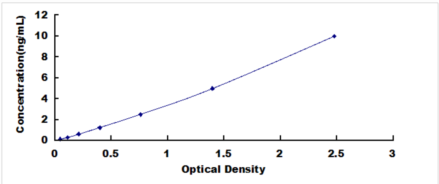
Typical Standard Curve for KRT7, Human ELISA.
