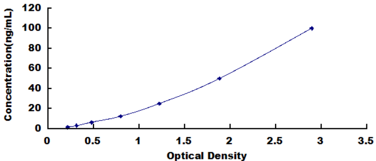
Typical Standard Curve for DEFa1, Mouse ELISA.
