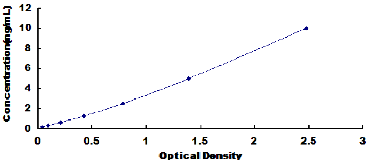
Typical Standard Curve for DNASEX, Human ELISA.
