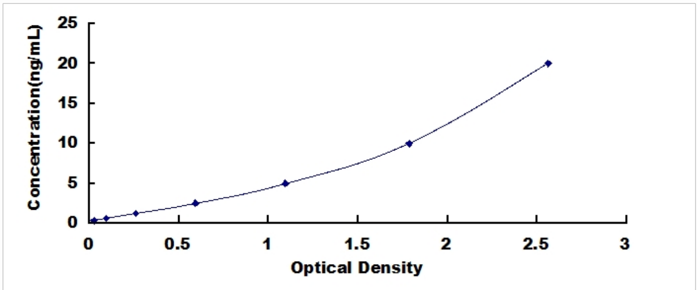
Typical Standard Curve for DSE, Human ELISA.
