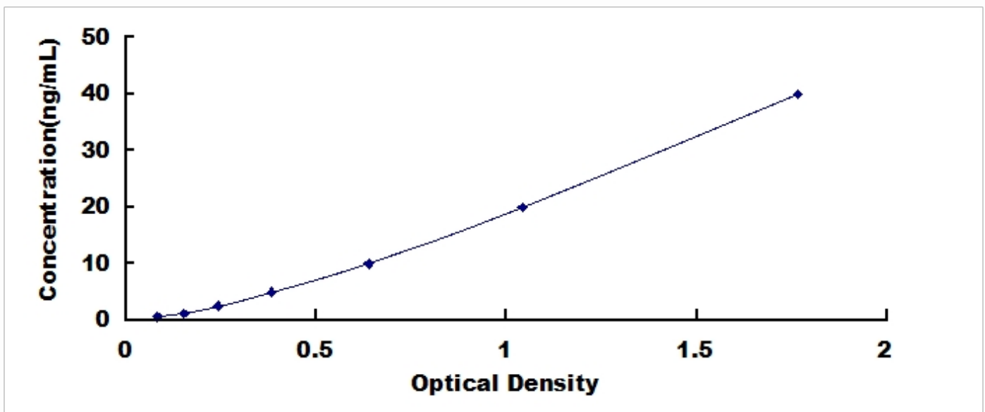
Typical Standard Curve for DAO, Rat ELISA.
