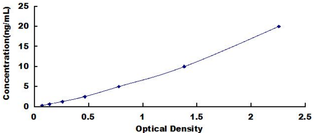
Typical Standard Curve for DRD3, Human ELISA.
