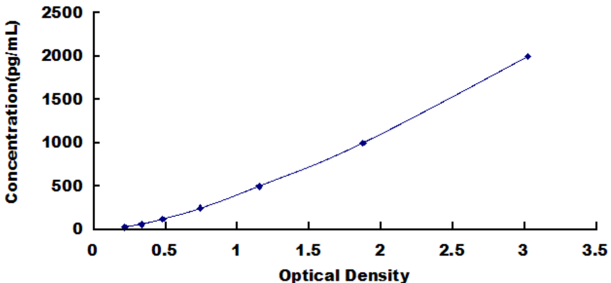
Typical Standard Curve for DUSP1, Mouse ELISA.
