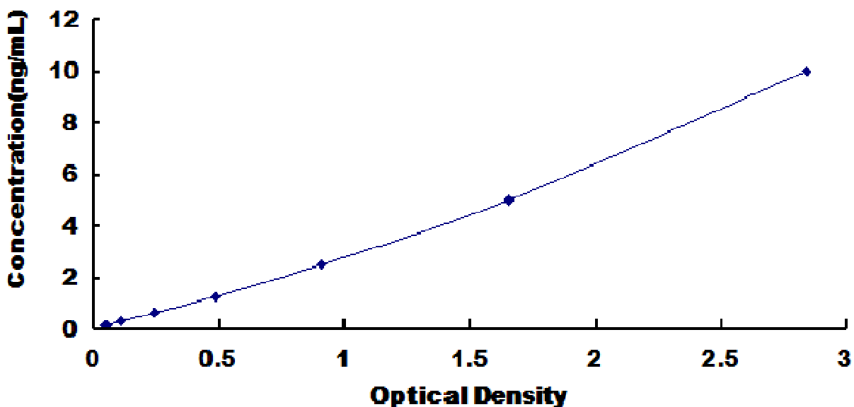
Typical Standard Curve for DUSP5, Human ELISA.
