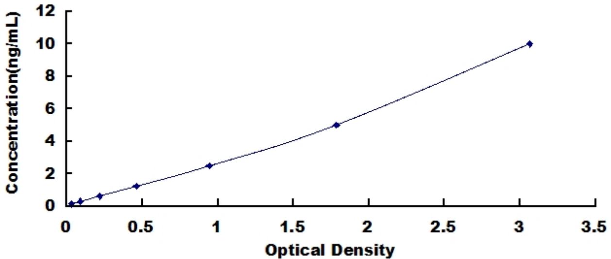
Typical Standard Curve for EDA2R, Human ELISA.
