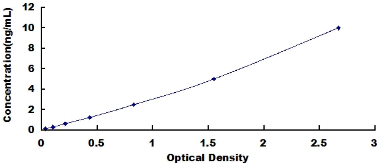
Typical Standard Curve for EZH2, Human ELISA.
