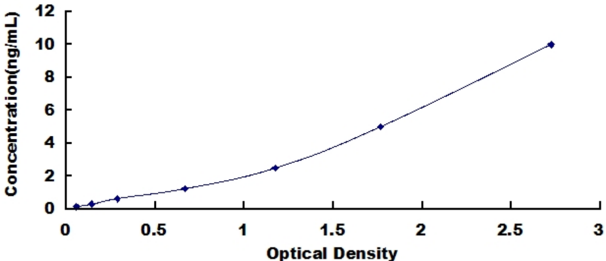
Typical Standard Curve for EPDR1, Human ELISA.
