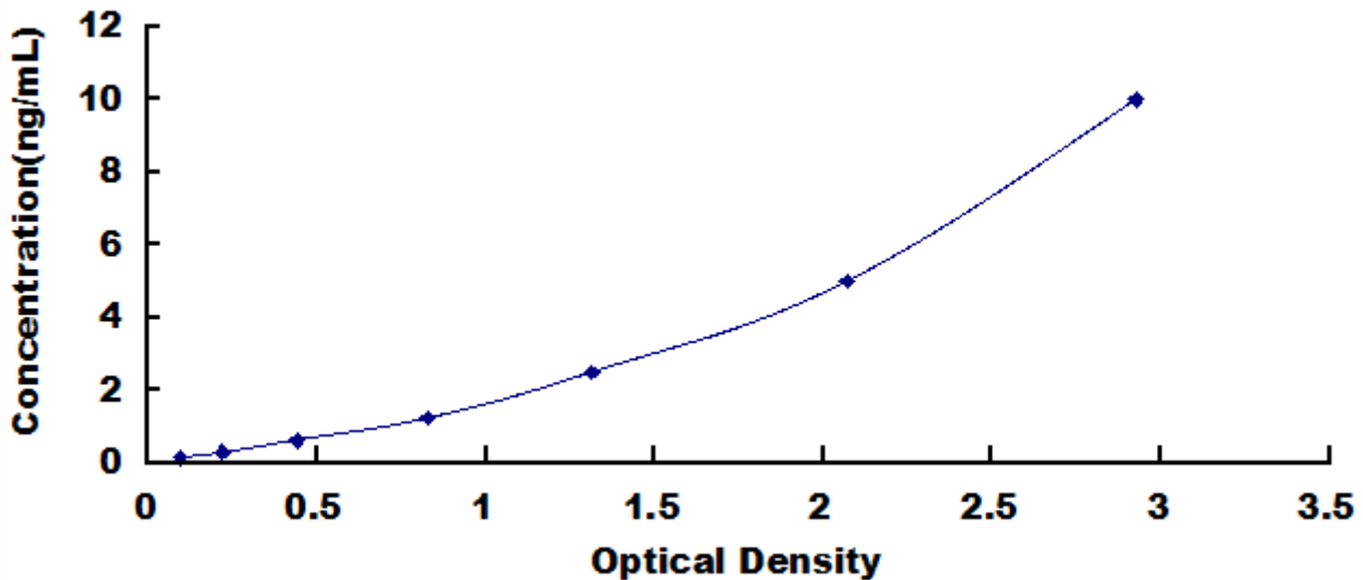
Typical Standard Curve for EEF1a1, Rat ELISA.
