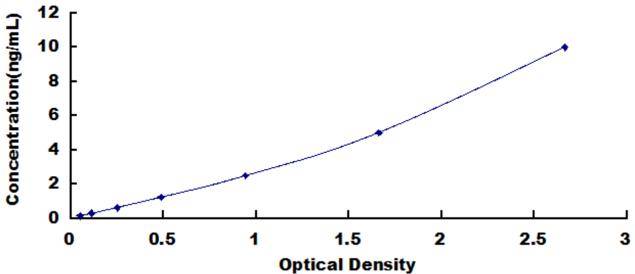
Typical Standard Curve for EIF2aK4, Human ELISA.
