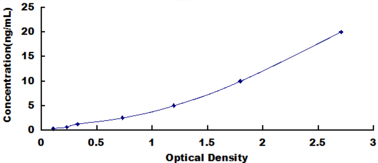
Typical Standard Curve for EAAT2, Human ELISA.
